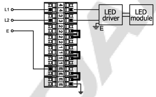
CIRCUIT DIAGRAM
